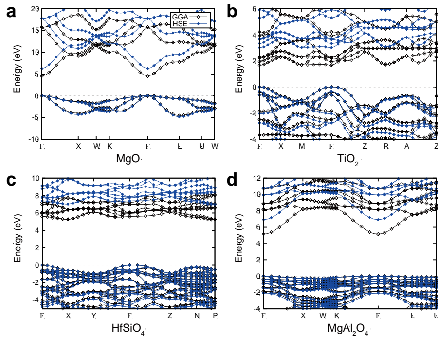
Figure S1. Comparison of GGA and HSE06 band structures for some oxides. The rigid shift between the bands are noticeable.
