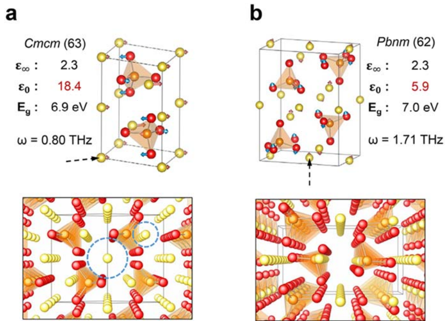
Figure S2. a) Cmcm and b) Pbnm phases of Na 2 SO 4 . The atomic arrangements viewed along the dashed arrows are shown at the bottom. The dashed circles in a) show the unblocked channel along which Na atoms can oscillate in large amplitudes.
