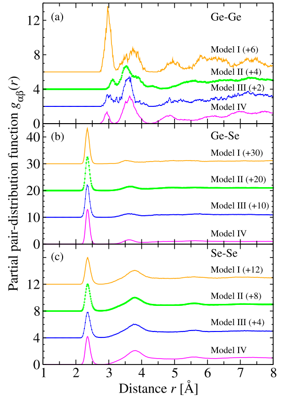
FIG. 5. The (a) Ge–Ge, (b) Ge–Se, and (c) Se–Se partial pair-distribution functions g_{\alpha\beta}(r) for glassy \text{GeSe}_9 from FPMD models I (solid orange curve), 22 II (broken green curve with squares), III (solid blue curve with squares), and IV (solid magenta curve). Several of the data sets have been shifted vertically for clarity of presentation.
