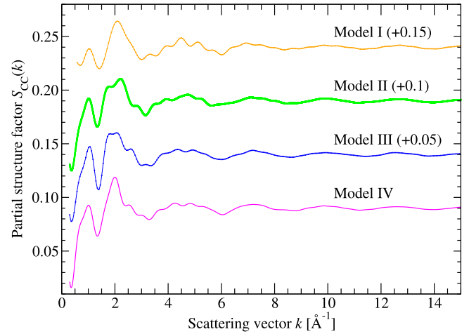
FIG. 3. The Bhatia-Thornton concentration-concentration partial structure factor S_{\text{CC}}(k) for glassy \text{GeSe}_9 from FPMD models I (solid orange curve), 22 II (broken green curve with squares), III (solid blue curve with squares), and IV (solid magenta curve). Several of the data sets have been shifted vertically for clarity of presentation.
