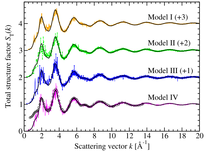
FIG. 1. The neutron total structure factor S_T(k) for glassy GeSe _9 . The measured S_T(k) function from the present work is given by the solid (black) curves with vertical error bars, where the size of the error bars is smaller than the line thickness at most k values, and the measured S_T(k) function from Ref. 39 is given by the (black) circles. The experimental results are compared to those obtained from FPMD models I (solid orange curve), 22 II (broken green curve with squares), III (solid blue curve with squares), and IV (solid magenta curve) by a direct calculation in reciprocal space. Several of the data sets have been shifted vertically for clarity of presentation.
