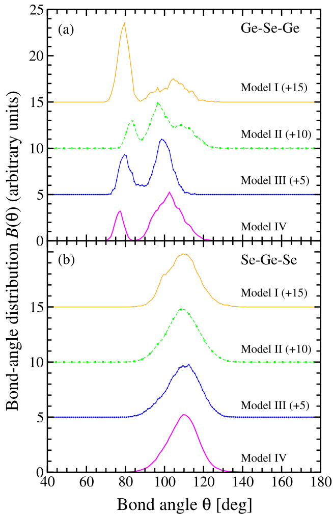
FIG. 6. The bond-angle distributions (a) B(\theta_{\text{GeSeGe}}) and (b) B(\theta_{\text{SeGeSe}}) for glassy \text{GeSe}_9 , where a cutoff distance r_{\text{cut}} = 2.75 \text{ \AA} was used in the analysis. The results correspond to FPMD models I (solid orange curve), 22 II (broken green curve with squares), III (solid blue curve with squares), and IV (solid magenta curve). Several of the data sets have been shifted vertically for clarity of presentation.
