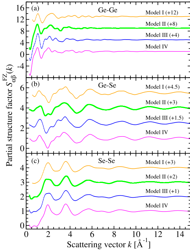
FIG. 2. The (a) Ge–Ge, (b) Ge–Se, and (c) Se–Se Faber-Ziman partial structure factors S_{\alpha\beta}^{\text{FZ}}(k) for glassy \text{GeSe}_9 from FPMD models I (solid orange curve), 22 II (broken green curve with squares), III (solid blue curve with squares), and IV (solid magenta curve). The functions were obtained by Fourier transforming the g_{\alpha\beta}(r) functions shown in Fig. 5. Several of the data sets have been shifted vertically for clarity of presentation.
