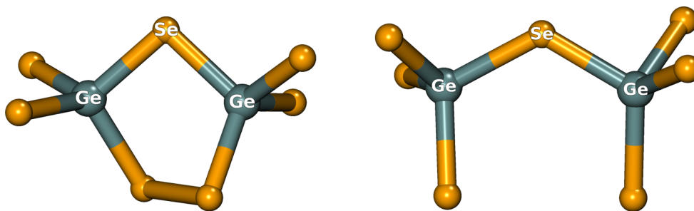
FIG. 7. The CS motifs in model II that lead to bi-modal CS features in both g_{\text{GeGe}}(r) (Fig. 5(a)) and B(\theta_{\text{SeGeSe}}) (Fig. 6(a)). The Ge and Se atoms are represented by the dark (blue) and light (golden) balls, respectively, and the bonds are represented by sticks. Fivefold ring conformations of the type shown in the left-hand panel lead to peaks at \sim 3.5 \text{ \AA} in g_{\text{GeGe}}(r) and at \sim 97^\circ in B(\theta_{\text{SeGeSe}}) . Conformations of the type shown in the right-hand panel lead to shoulders at \sim 3.8 \text{ \AA} in g_{\text{GeGe}}(r) and at \sim 109^\circ in B(\theta_{\text{SeGeSe}}) .
