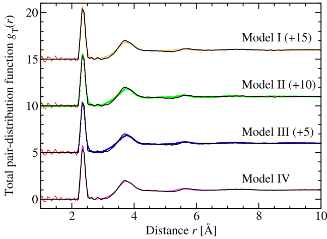
FIG. 4. The neutron total pair-distribution function g_T(r) for glassy \text{GeSe}_9 . The measured g_T(r) function from the present work [solid (black) curves] was obtained by Fourier transforming the spline-fitted measured S_T(k) function shown in Fig. 1 with k_{\text{max}} = 30 \text{ \AA}^{-1} . The Fourier transform artifacts at r values smaller than the distance of closest approach between two atoms are shown by the chained (red) curves. The experimental results are compared to those obtained from FPMD models I (solid orange curve), 22 II (broken green curve with squares), III (solid blue curve with squares), and IV (solid magenta curve). Several of the data sets have been shifted vertically for clarity of presentation.
